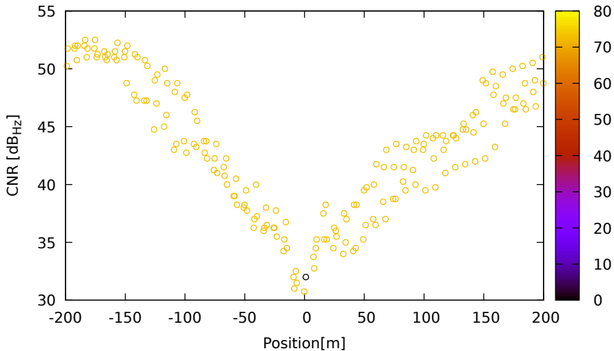
CNR vs position for E19 (E5) on LeicaGS18 - DOY 263 jam. 1
