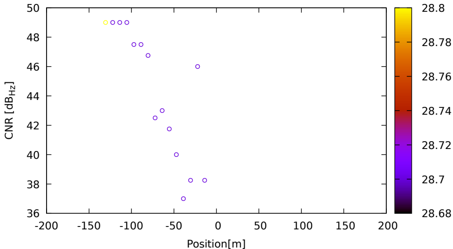
CNR vs position for E33 (E1) on LeicaGS18 - DOY 263 jam. 3
