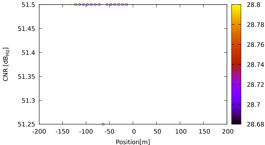
CNR vs position for E33 (E5) on LeicaGS18 - DOY 263 jam. 3
