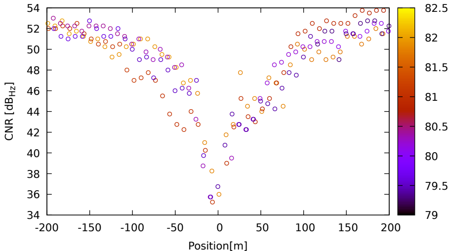
CNR vs position for G01 (L1) on LeicaGS18 - DOY 263 jam. 1
