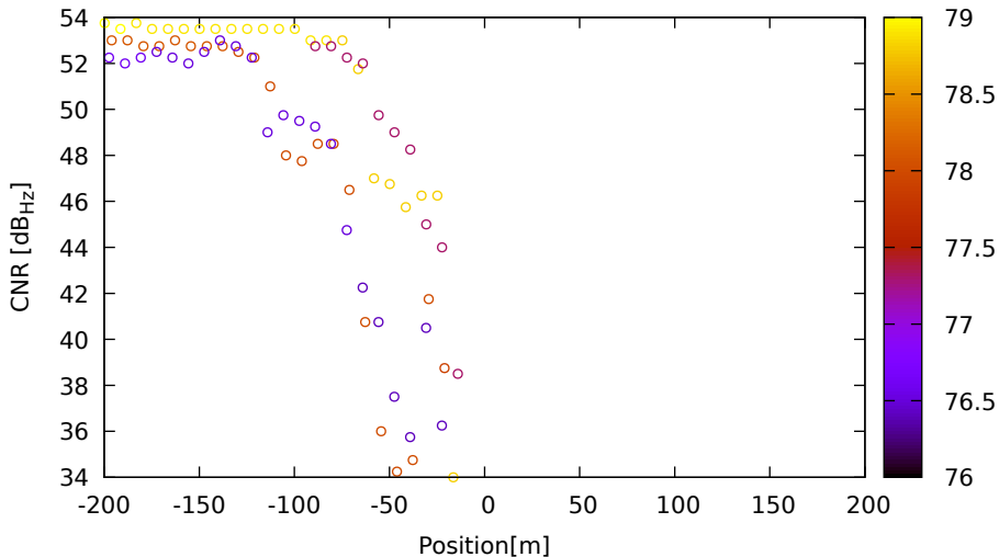
CNR vs position for G01 (L1) on LeicaGS18 - DOY 263 jam. 2
