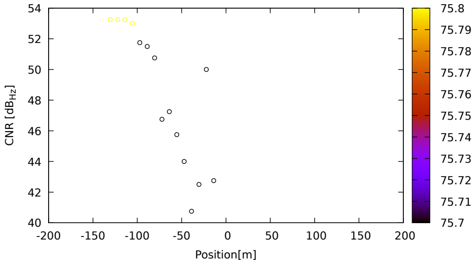
CNR vs position for G01 (L1) on LeicaGS18 - DOY 263 jam. 3
