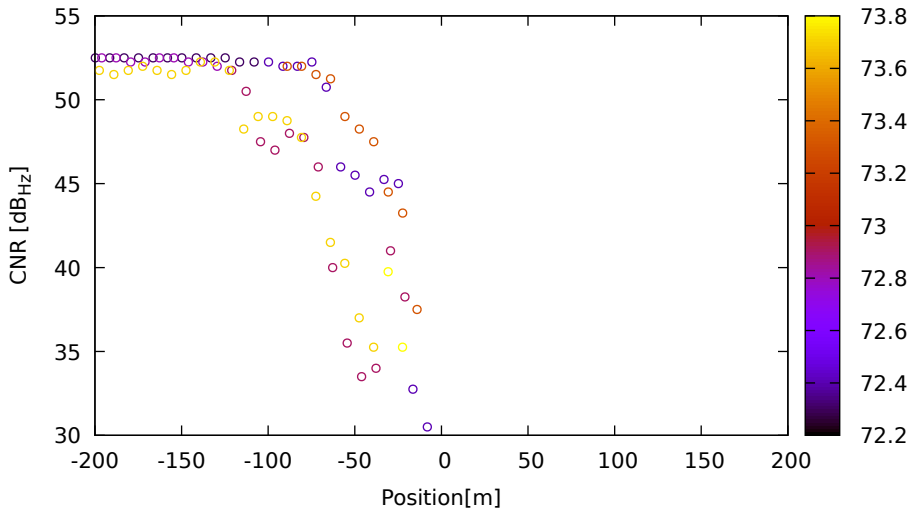
CNR vs position for G03 (L1) on LeicaGS18 - DOY 263 jam. 2
