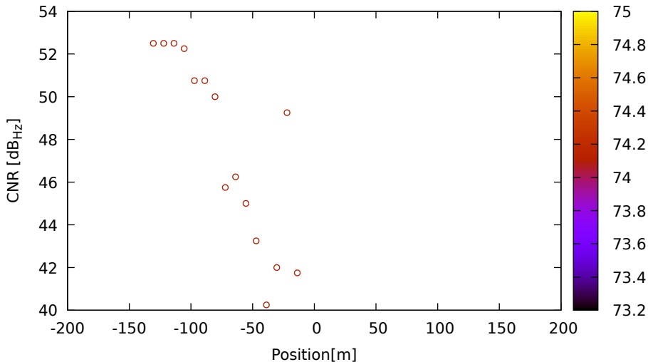
CNR vs position for G03 (L1) on LeicaGS18 - DOY 263 jam. 3
