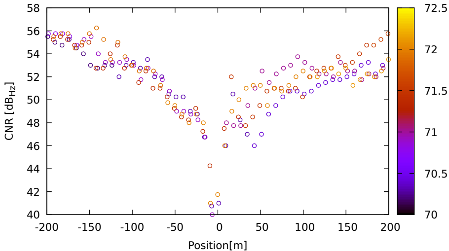
CNR vs position for G03 (L5) on LeicaGS18 - DOY 263 jam. 1
