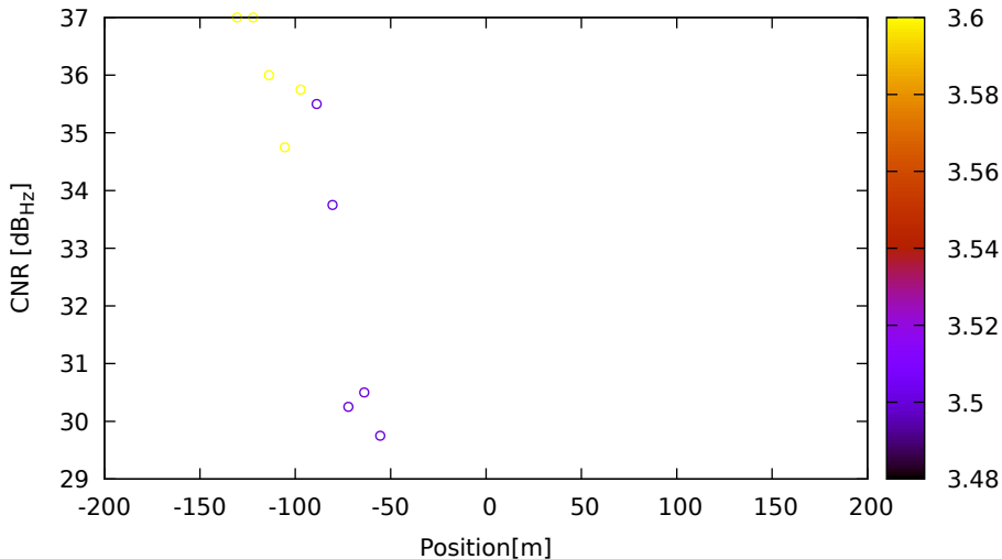
CNR vs position for G08 (L2) on LeicaGS18 - DOY 263 jam. 3
