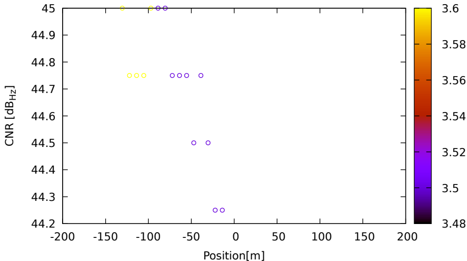
CNR vs position for G08 (L5) on LeicaGS18 - DOY 263 jam. 3
