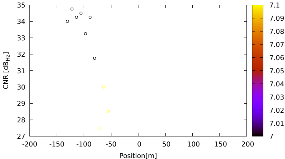
CNR vs position for G09 (L2) on LeicaGS18 - DOY 263 jam. 3
