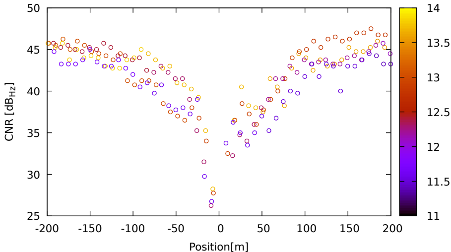
CNR vs position for G32 (L2) on LeicaGS18 - DOY 263 jam. 1
