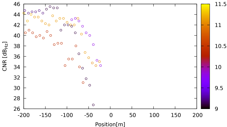
CNR vs position for G32 (L2) on LeicaGS18 - DOY 263 jam. 2
