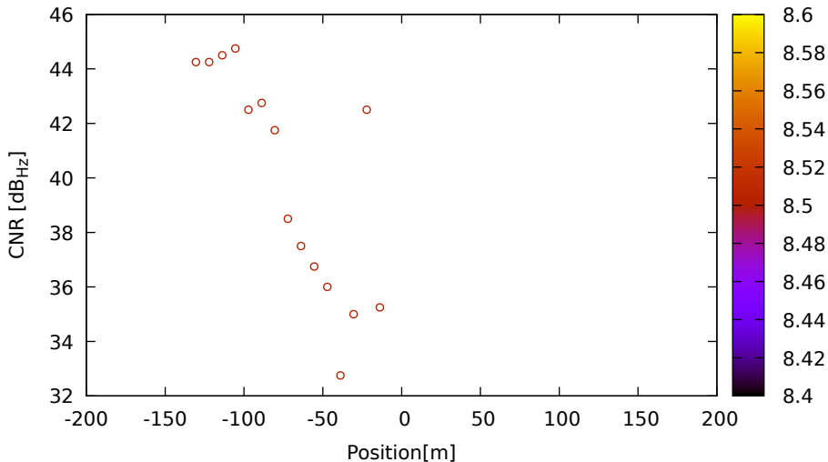
CNR vs position for G32 (L2) on LeicaGS18 - DOY 263 jam. 3
