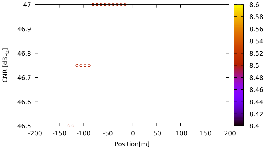
CNR vs position for G32 (L5) on LeicaGS18 - DOY 263 jam. 3
