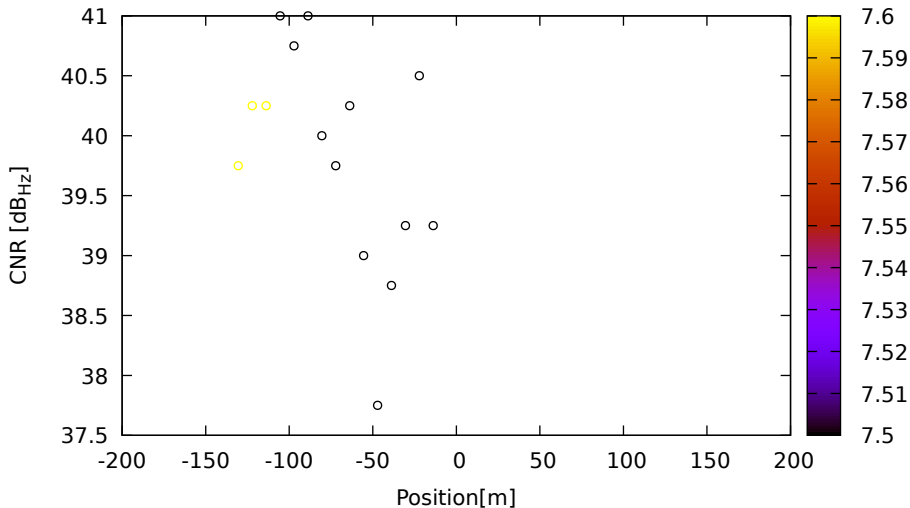
CNR vs position for R08 (G1) on LeicaGS18 - DOY 263 jam. 3
