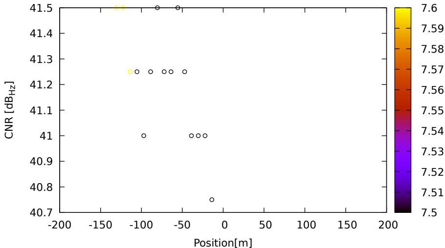
CNR vs position for R08 (G2) on LeicaGS18 - DOY 263 jam. 3
