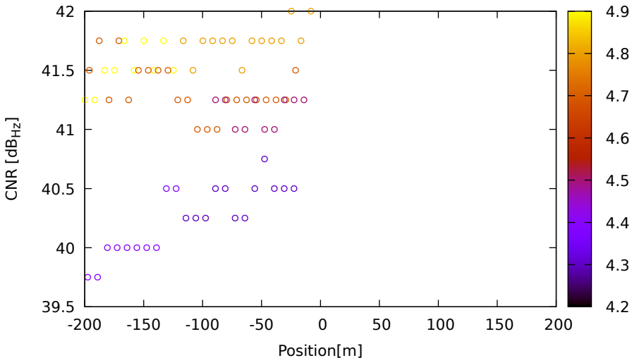
CNR vs position for R09 (G2) on LeicaGS18 - DOY 263 jam. 2
