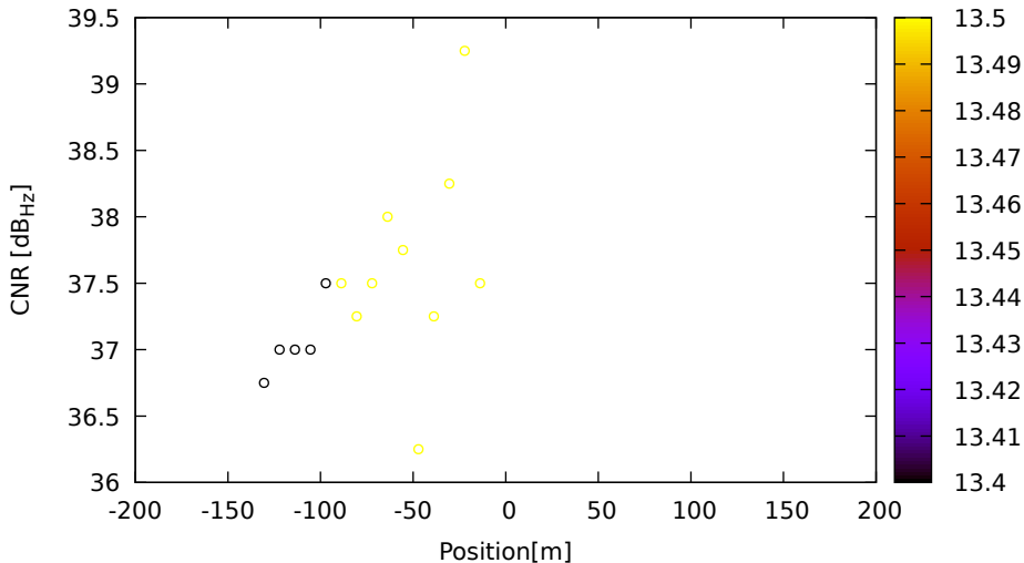
CNR vs position for R18 (G1) on LeicaGS18 - DOY 263 jam. 3
