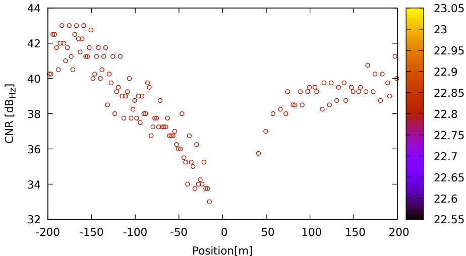
CNR vs position for C05 (B2) on LeicaGS18 - DOY 263 jam. 1
