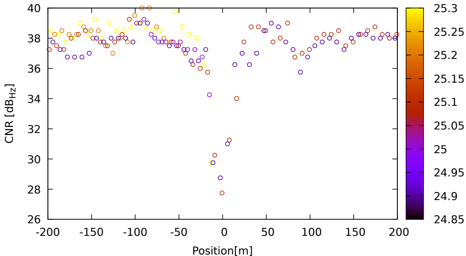
CNR vs position for C16 (B3) on LeicaGS18 - DOY 263 jam. 1
