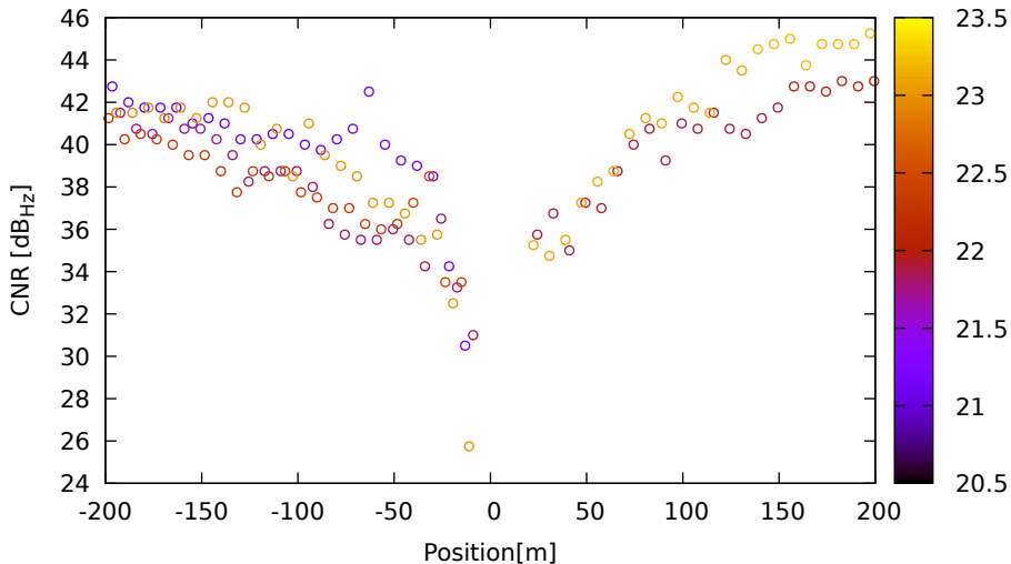
CNR vs position for C33 (B1) on LeicaGS18 - DOY 263 jam. 1
