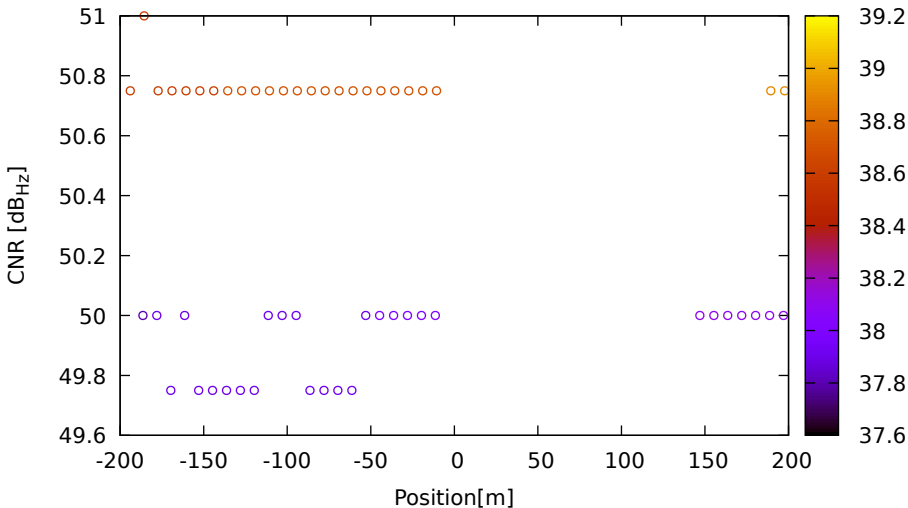
CNR vs position for E04 (E5a) on LeicaGS18 - DOY 263 jam. 3
