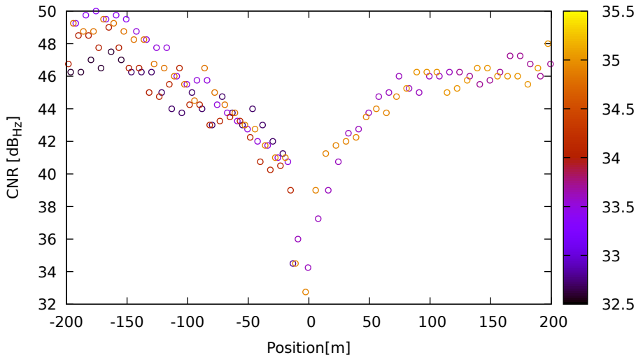
CNR vs position for E04 (E5b) on LeicaGS18 - DOY 263 jam. 1
