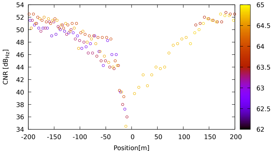
CNR vs position for E10 (E1) on LeicaGS18 - DOY 263 jam. 1
