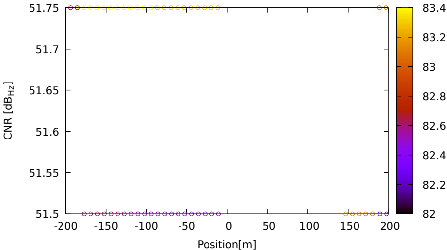
CNR vs position for E12 (E5b) on LeicaGS18 - DOY 263 jam. 3
