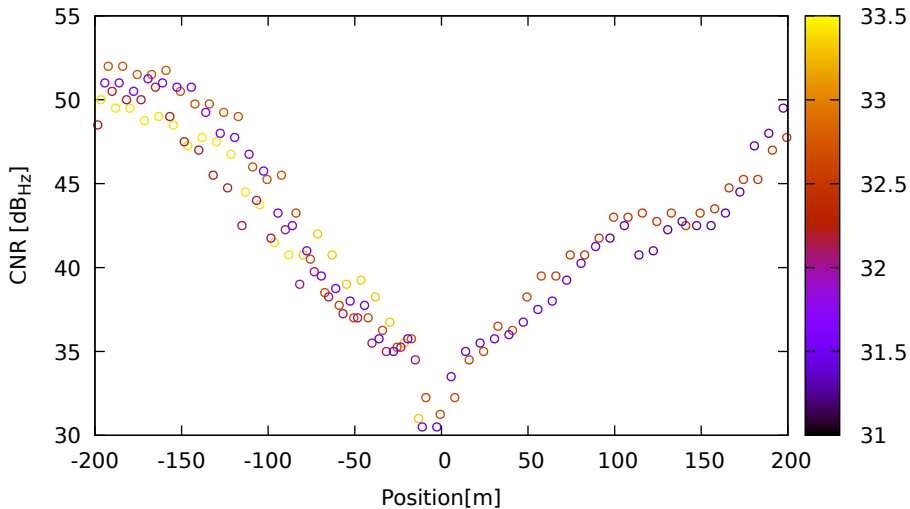
CNR vs position for E33 (E5) on LeicaGS18 - DOY 263 jam. 1
