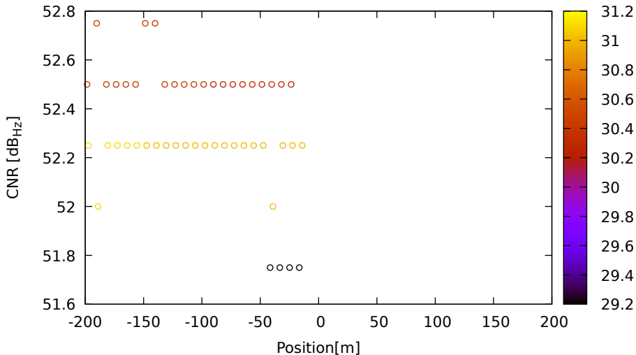
CNR vs position for E33 (E5) on LeicaGS18 - DOY 263 jam. 2
