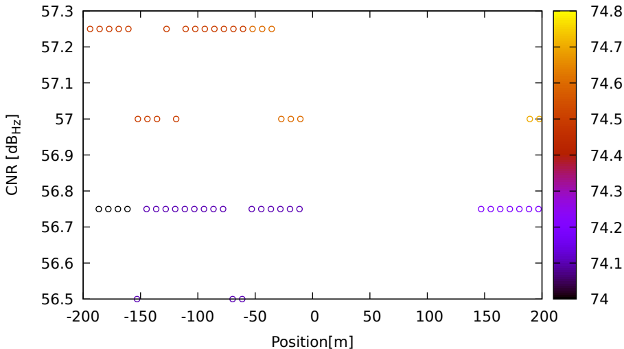
CNR vs position for G03 (L5) on LeicaGS18 - DOY 263 jam. 3
