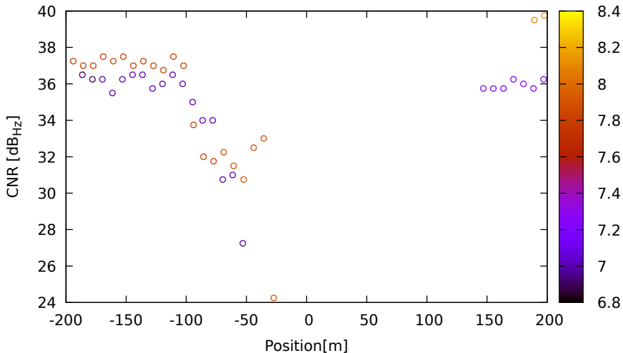
CNR vs position for G09 (L1) on LeicaGS18 - DOY 263 jam. 3
