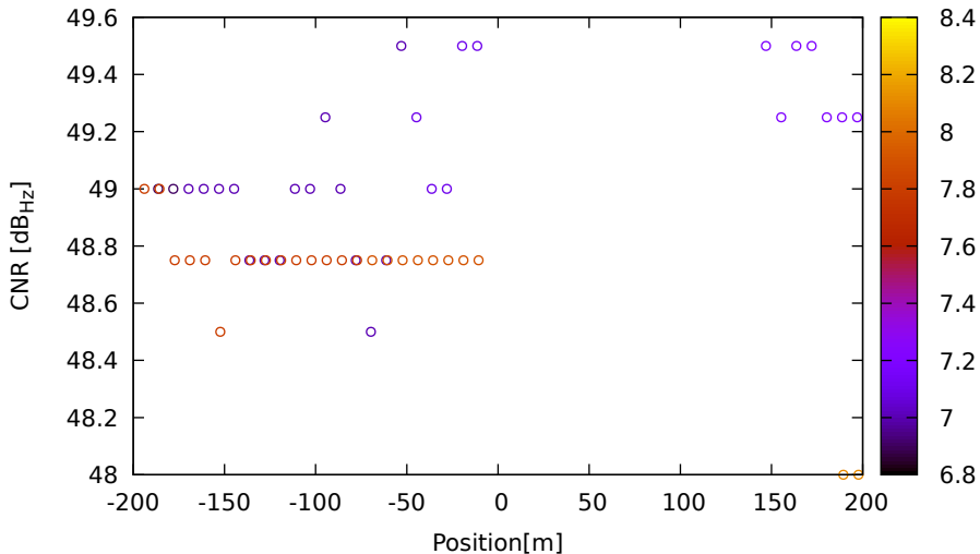
CNR vs position for G09 (L5) on LeicaGS18 - DOY 263 jam. 3
