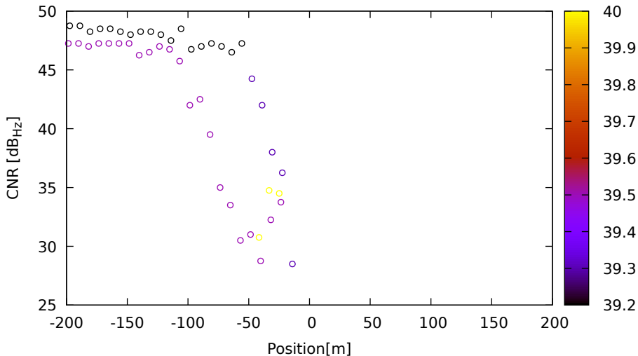
CNR vs position for G17 (L2) on LeicaGS18 - DOY 263 jam. 2
