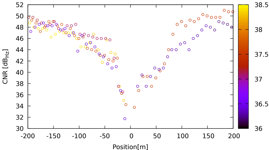
CNR vs position for G22 (L1) on LeicaGS18 - DOY 263 jam. 1
