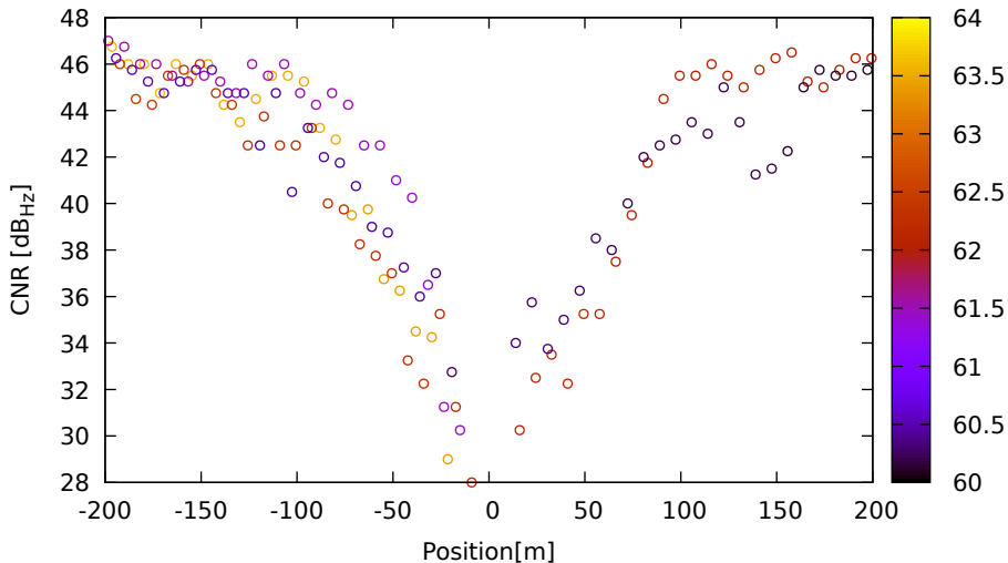
CNR vs position for R01 (G1) on LeicaGS18 - DOY 263 jam. 1
