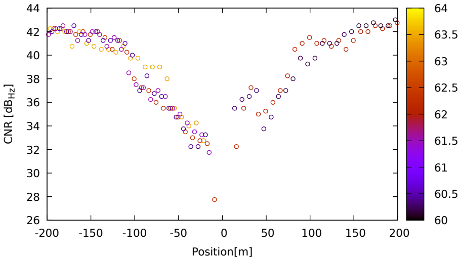
CNR vs position for R01 (G2) on LeicaGS18 - DOY 263 jam. 1
