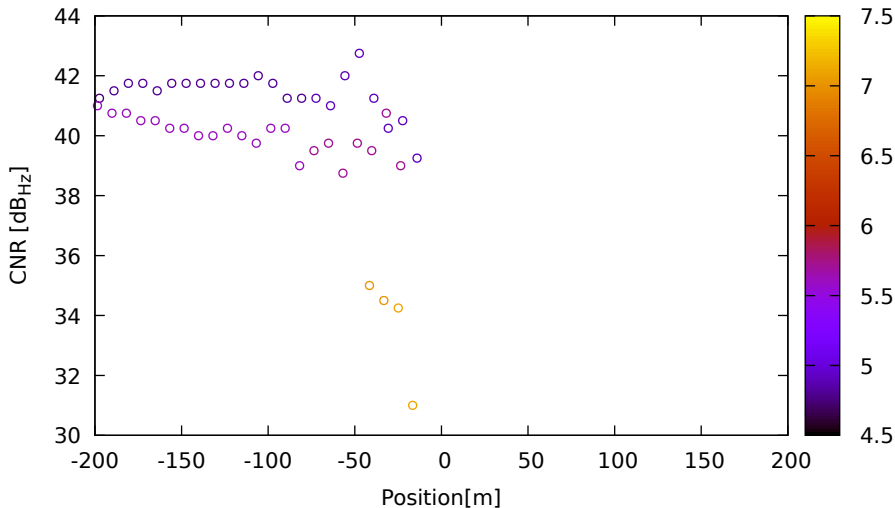
CNR vs position for R03 (G1) on LeicaGS18 - DOY 263 jam. 2
