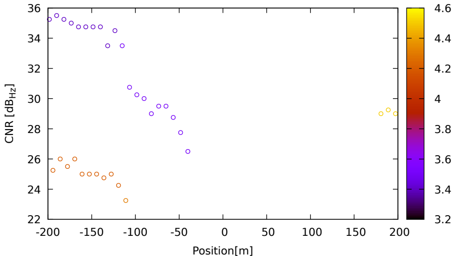
CNR vs position for R03 (G2) on LeicaGS18 - DOY 263 jam. 1
