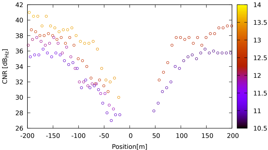
CNR vs position for R08 (G2) on LeicaGS18 - DOY 263 jam. 1
