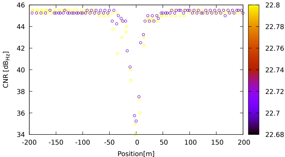
CNR vs position for C05 (B1) on SamsungS20 - DOY 263 jam. 2
