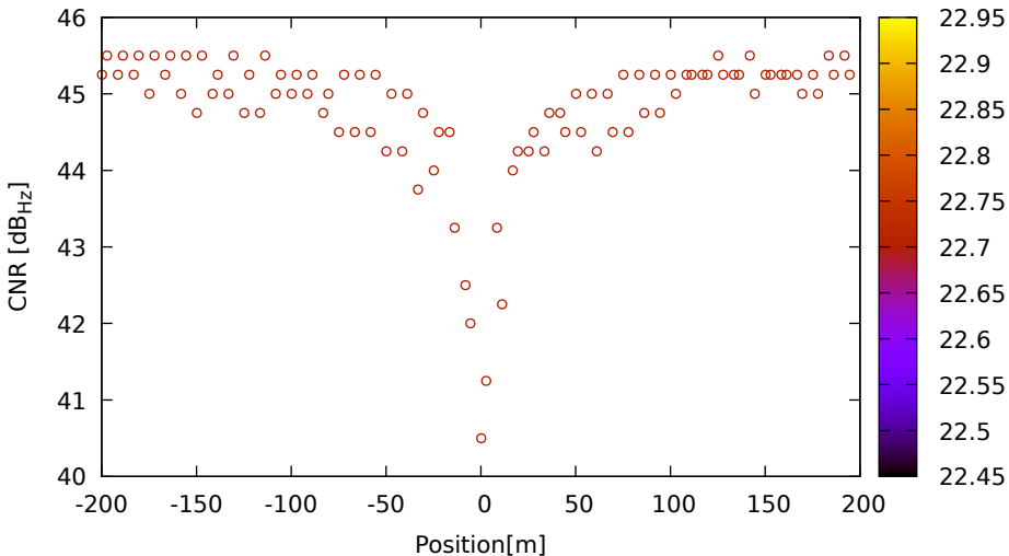
CNR vs position for C05 (B1) on SamsungS20 - DOY 263 jam. 3
