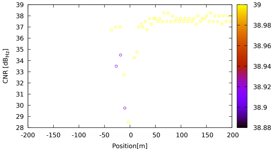
CNR vs position for C09 (B1) on SamsungS20 - DOY 263 jam. 2
