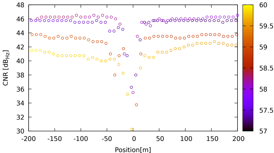
CNR vs position for C11 (B1) on SamsungS20 - DOY 263 jam. 2
