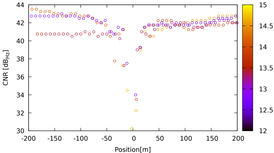
CNR vs position for C12 (B1) on SamsungS20 - DOY 263 jam. 2
