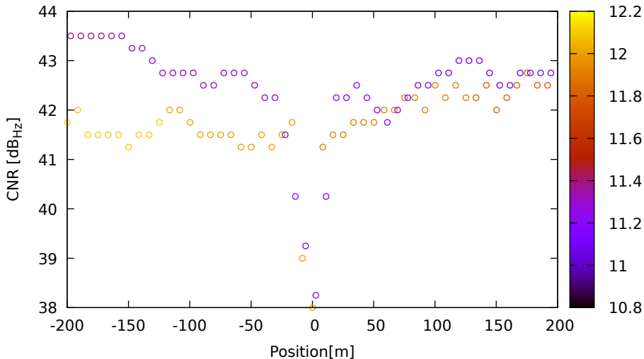
CNR vs position for C12 (B1) on SamsungS20 - DOY 263 jam. 3
