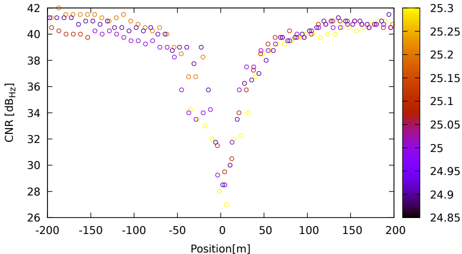
CNR vs position for C16 (B1) on SamsungS20 - DOY 263 jam. 1
