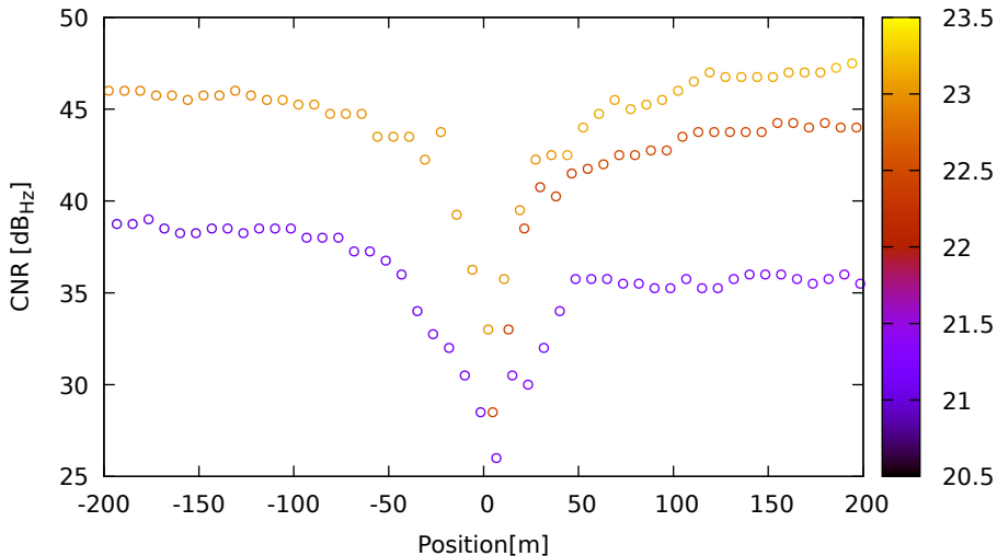
CNR vs position for C33 (B1) on SamsungS20 - DOY 263 jam. 1
