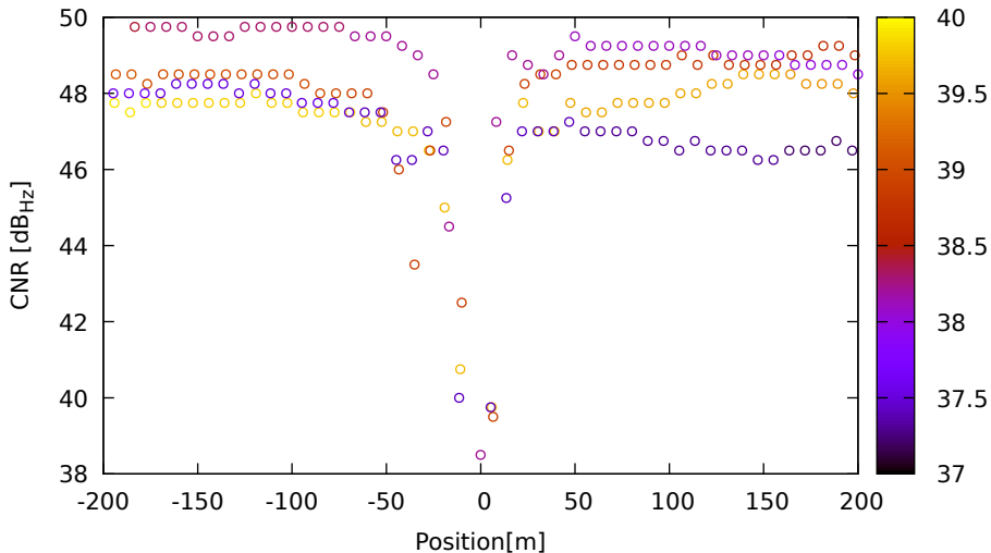
CNR vs position for C34 (B1) on SamsungS20 - DOY 263 jam. 2
