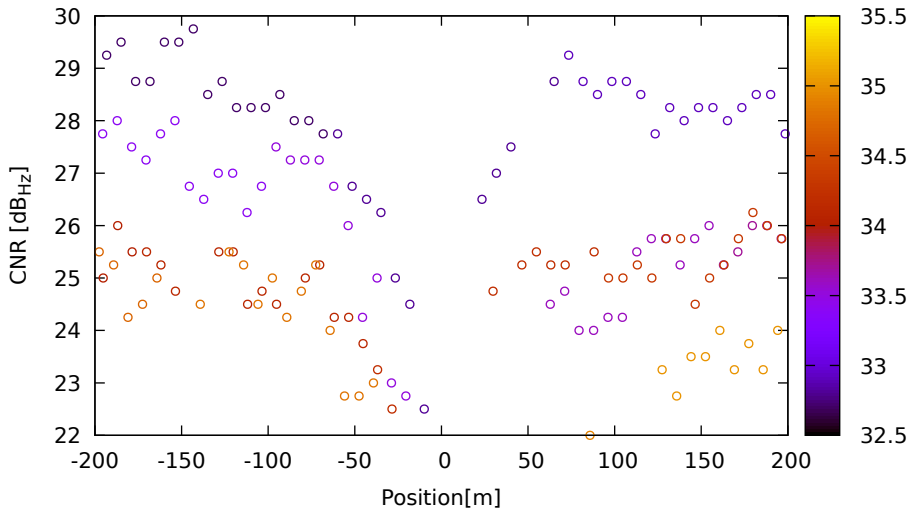
CNR vs position for E04 (E5a) on SamsungS20 - DOY 263 jam. 1
