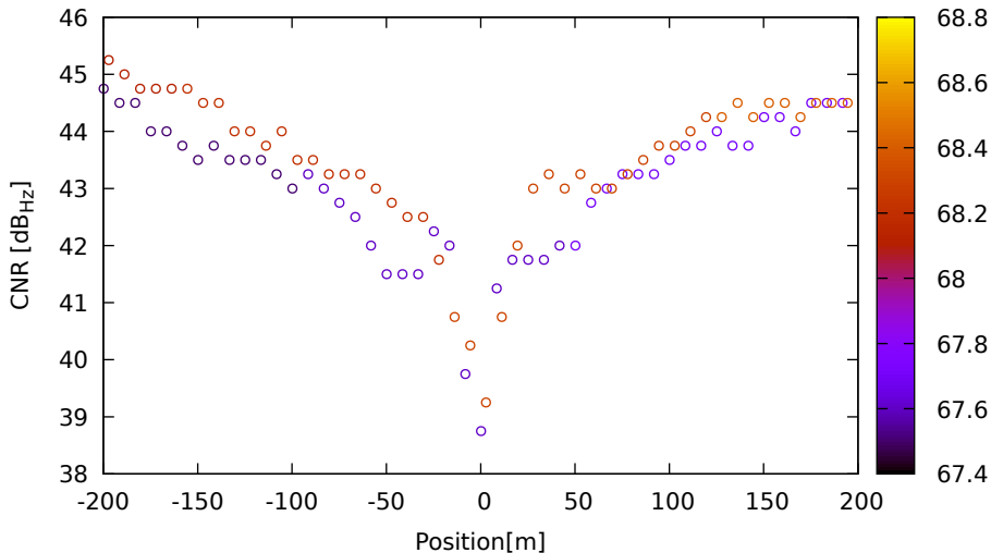
CNR vs position for E10 (E1) on SamsungS20 - DOY 263 jam. 3
